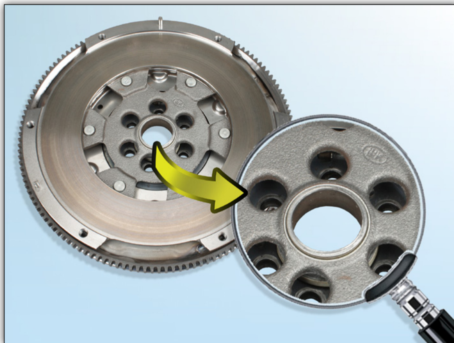
Image 1: LuK DMF 415 0059 10 with slide bearing
