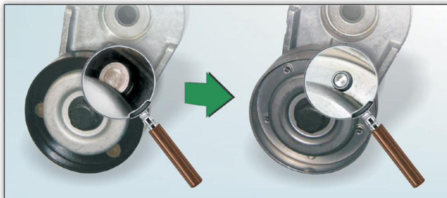
Image 1: Detailed view of pulley in its previous design (left) and new design (right)
