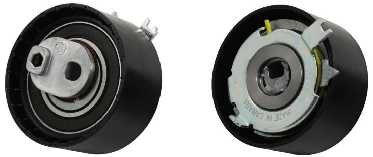
Image 1: INA tensioner pulley 531 0710 10
