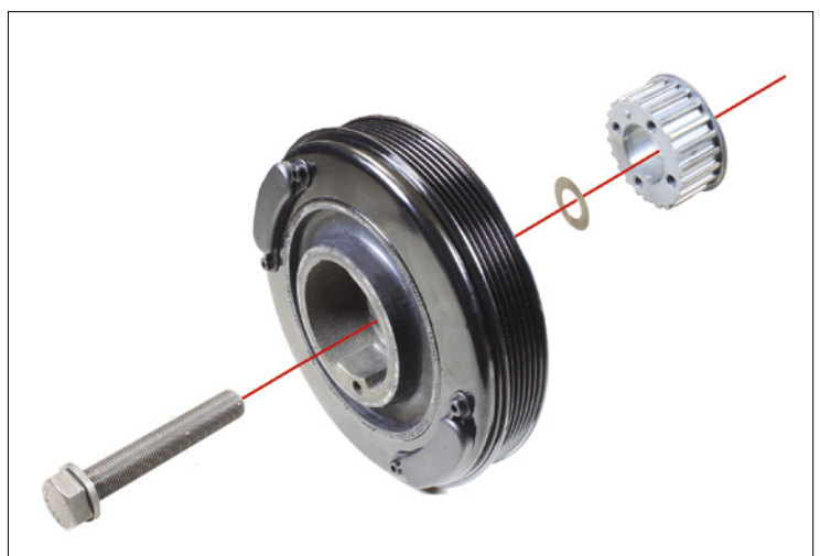
Image 1: crankshaft vibration damper with crankshaft central bolt and diamond washer
