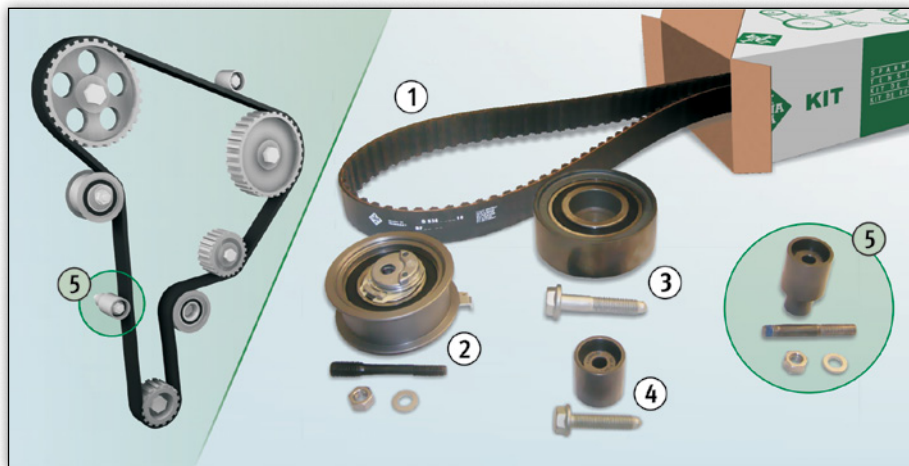
Image 1: Drive diagram 1.9 TDI/SDI and package content for KIT 530 0361 10/530 0082 10
